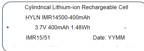
Label 2 for model HYLN IMR14500-400mAh
