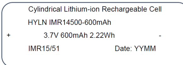
Label 4 for model HYLN IMR14500-600mAh
