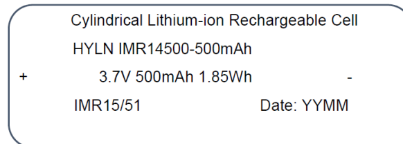
Label 3 for model HYLN IMR14500-500mAh
