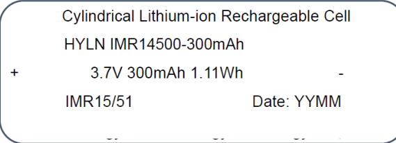
Label 1 for model HYLN IMR14500-300mAh
