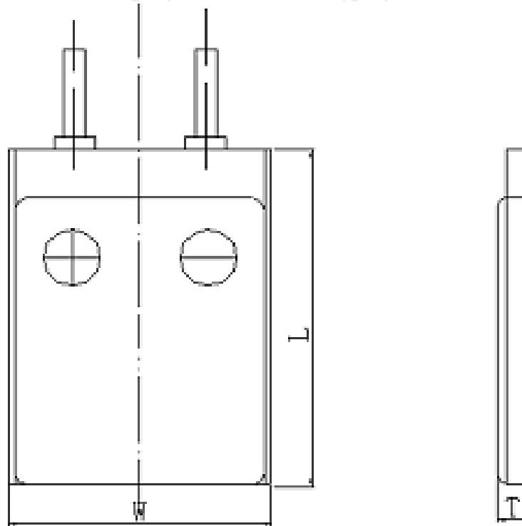
T: 3.4mm max W: 14.5mm max L: 23.5mm max Cell
