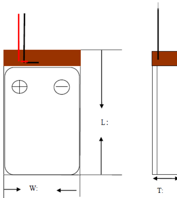
T: 3.4mm max W: 14.5mm max L: 24.2mm max Battery
