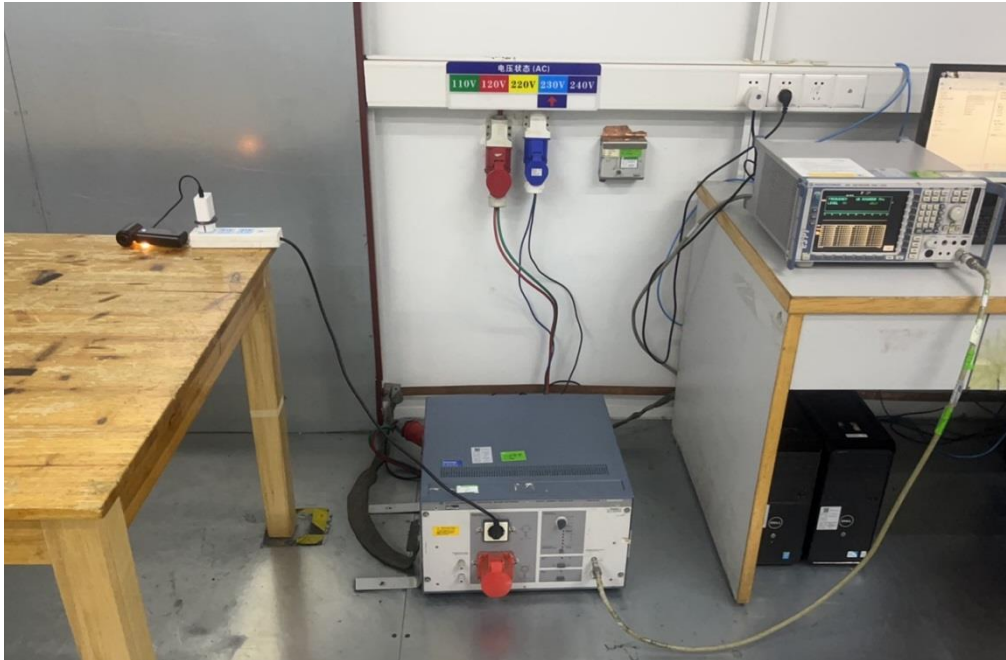
Conducted emissions from the AC mains power ports
