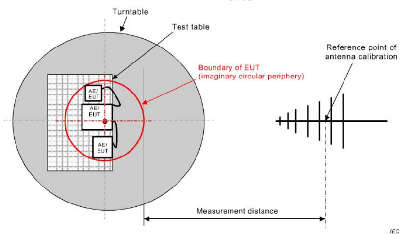
Figure C.1 – Measurement distance
