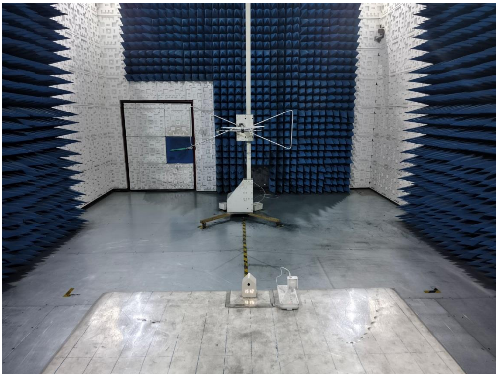
Radiated emissions at frequencies up to 1 GHz - Test Model: MO2730
