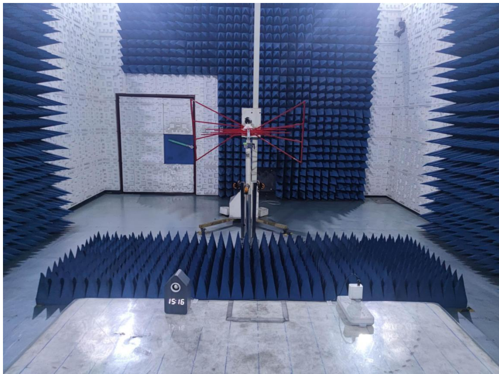
Radio-frequency electromagnetic field up to 1 GHz - Series Model(s): MO2731
