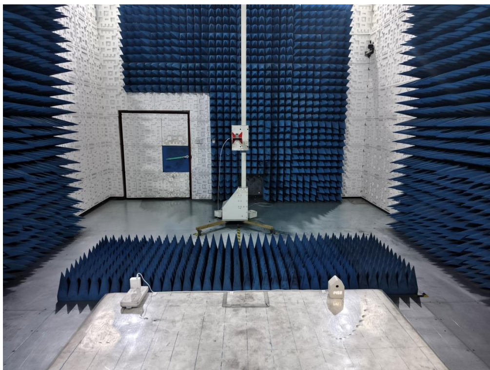
Radio-frequency electromagnetic field above 1 GHz - Test Model: MO2730
