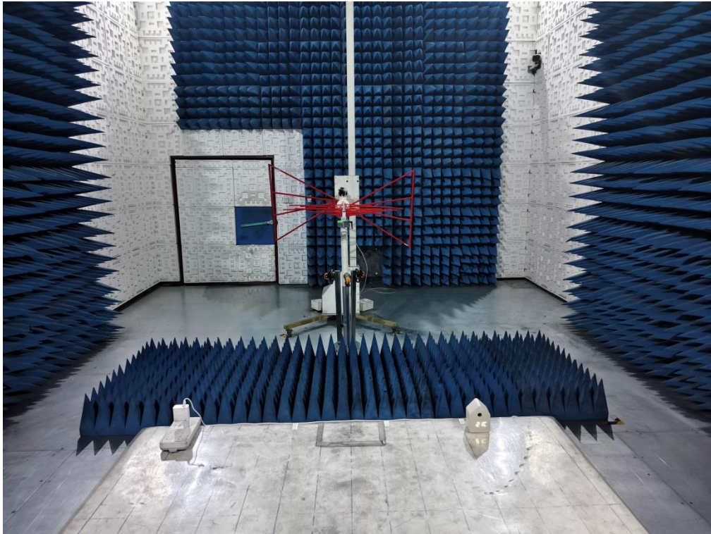
Radio-frequency electromagnetic field up to 1 GHz - Test Model: MO2730
