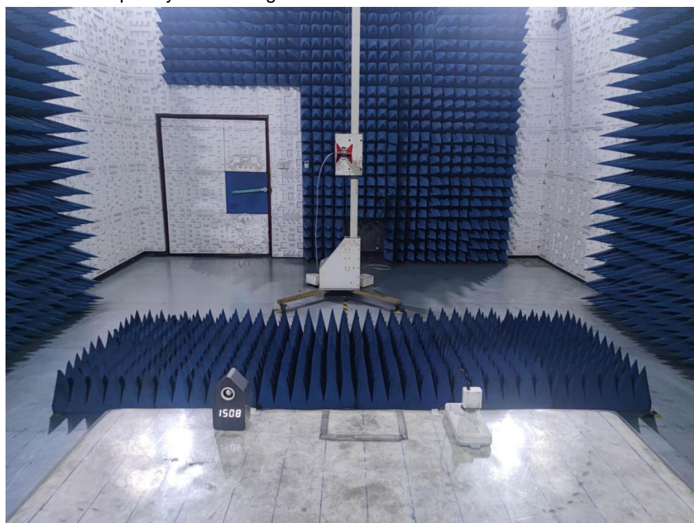
Radio-frequency electromagnetic field above 1 GHz - Series Model(s): MO2731
