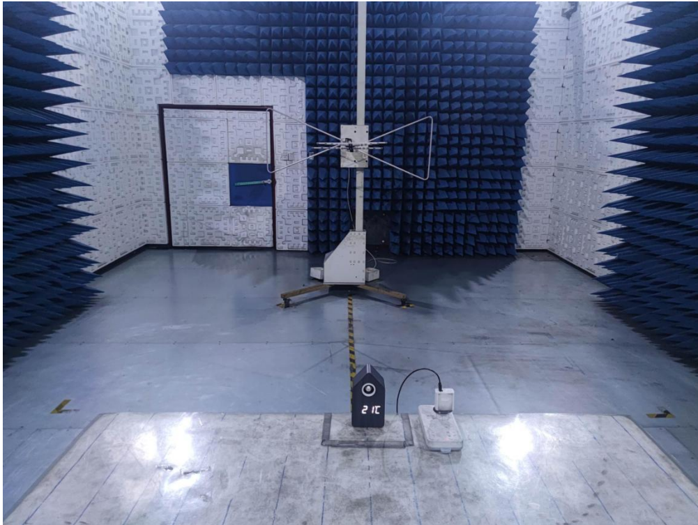
Radiated emissions at frequencies up to 1 GHz - Series Model(s): MO2731
