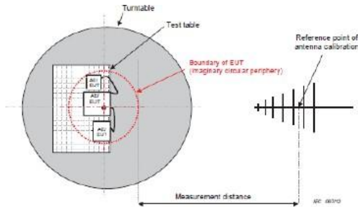
Figure C.1 – Measurement distance
