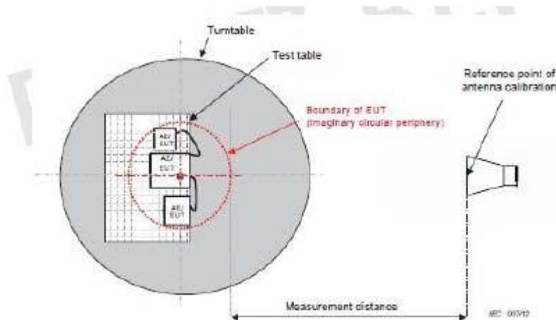
Figure C.1 – Measurement distance
