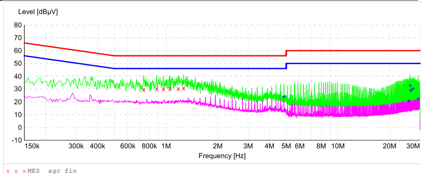
Test graph and data for Conducted Emission
