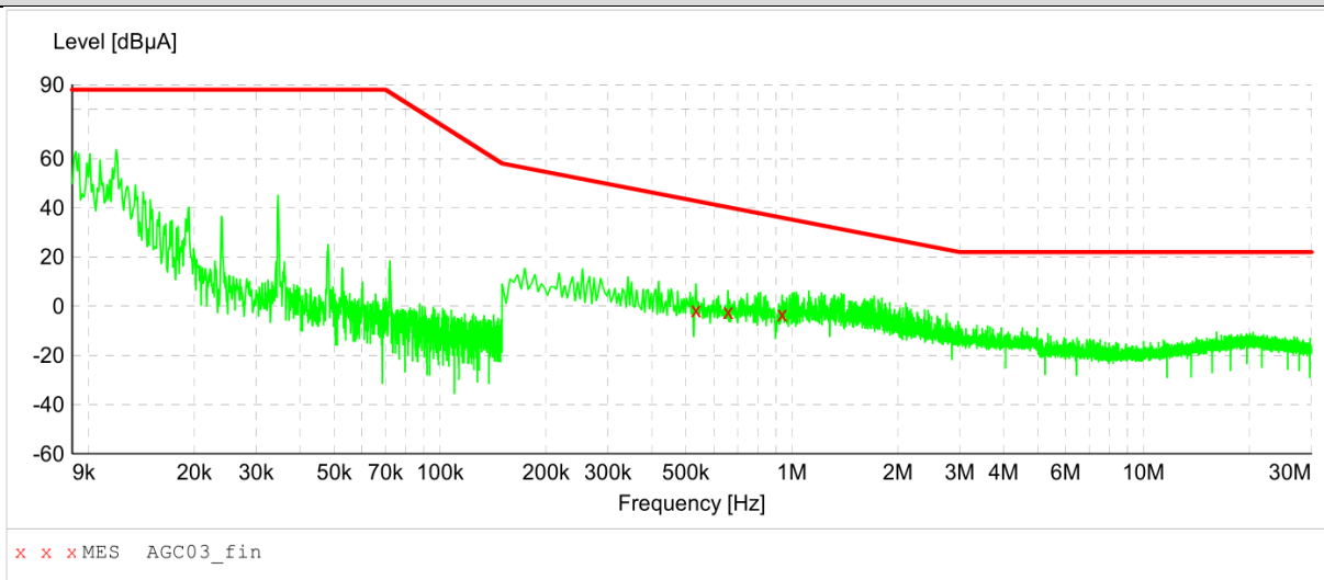
Test graph and data for LLAS radiated disturbance at loop X
