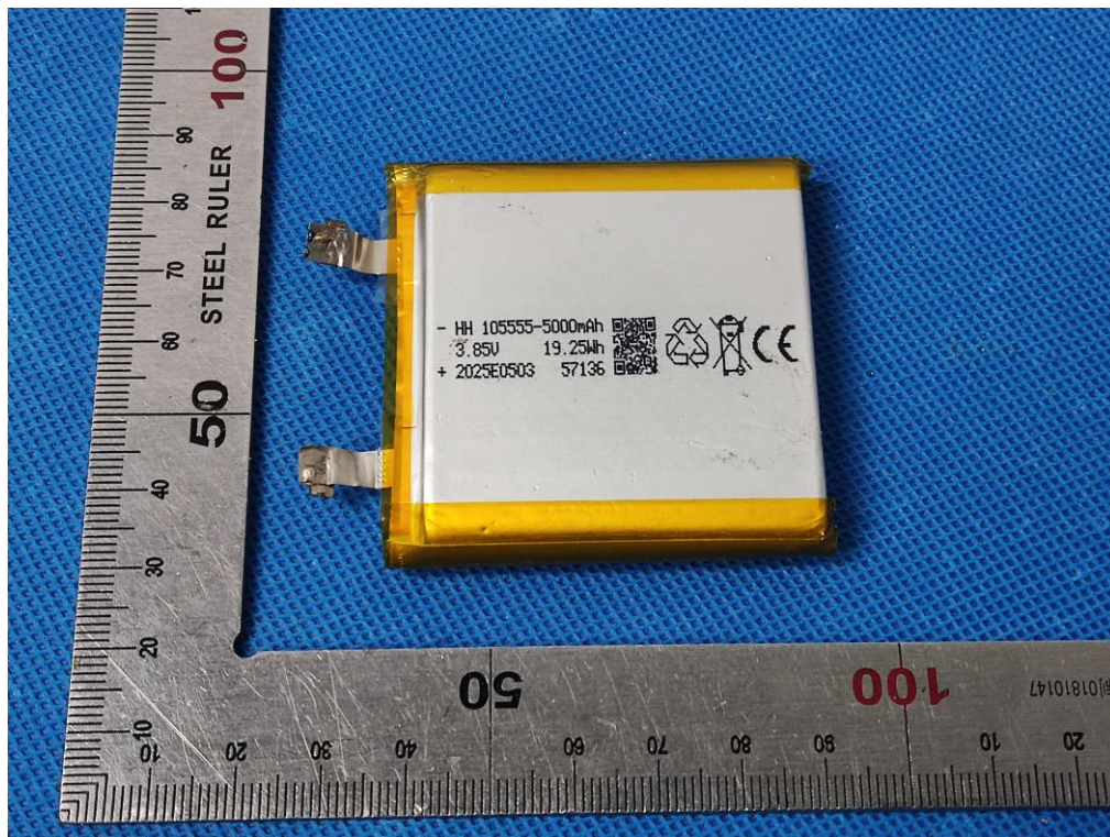
Fig. 7 –Battery cell view
