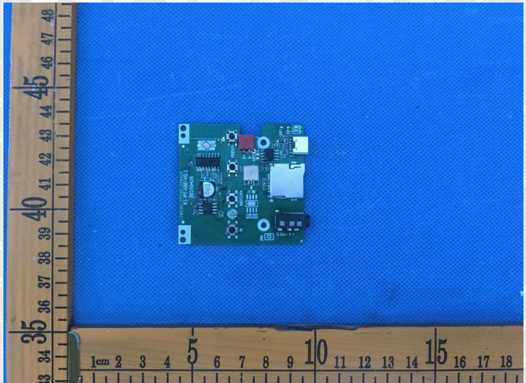
Figure 4: PCB view
