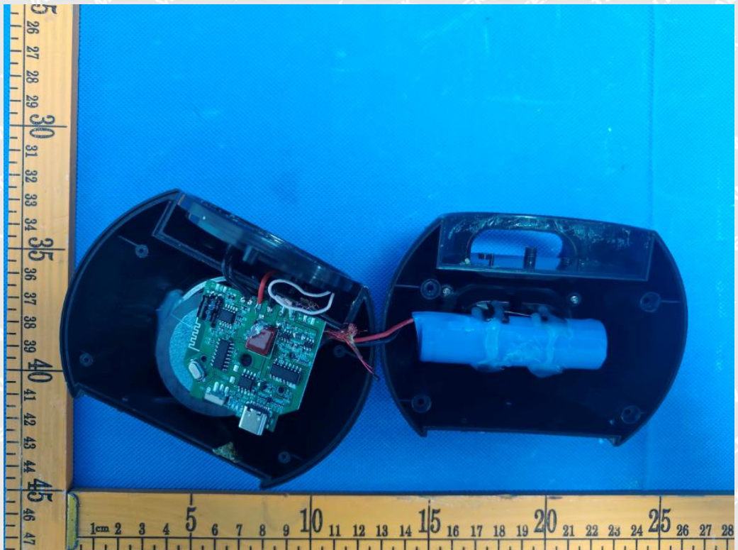
Figure 4: Internal view
