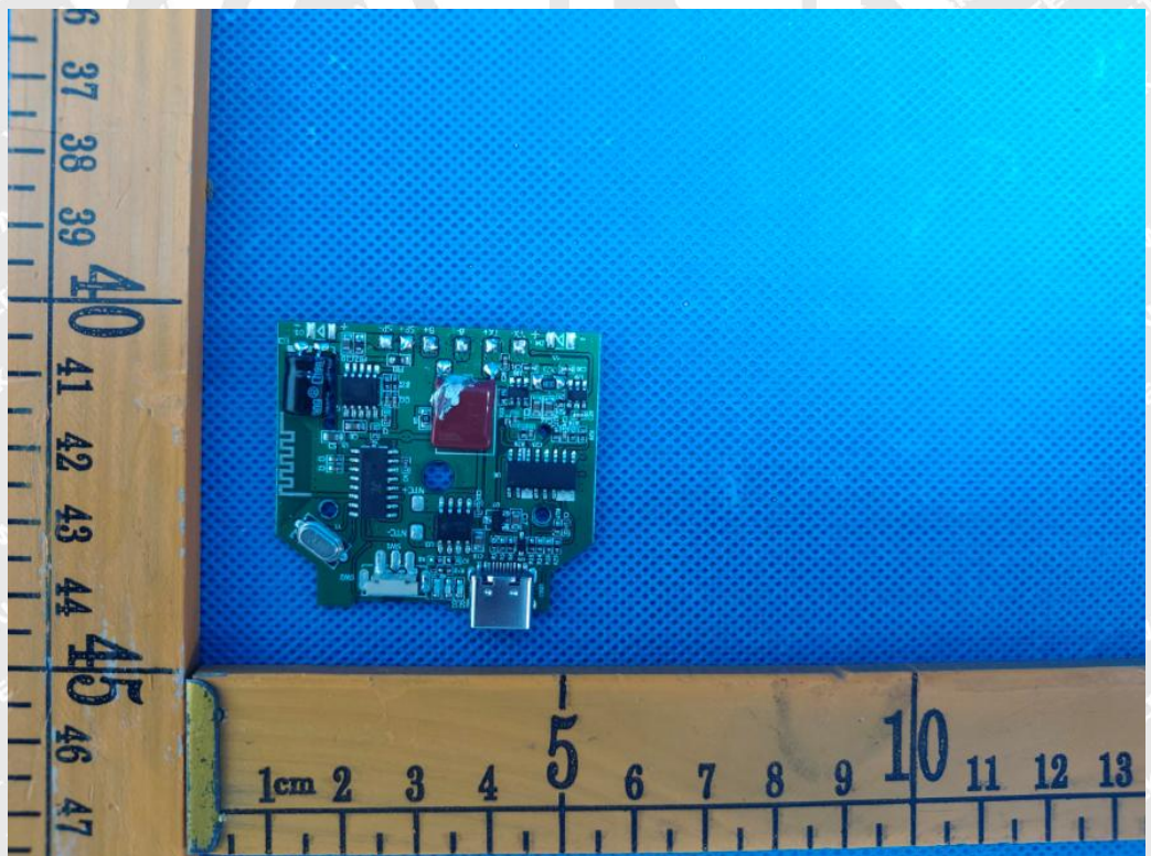
Figure 6: PCB view
