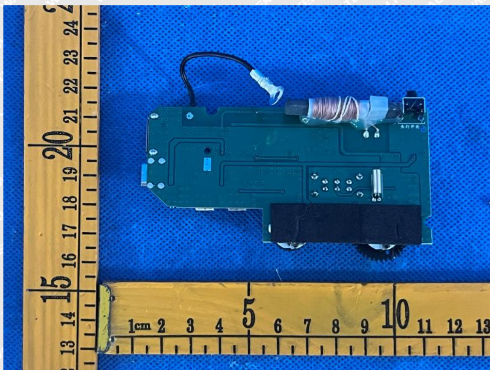
Figure 7: PCB view
