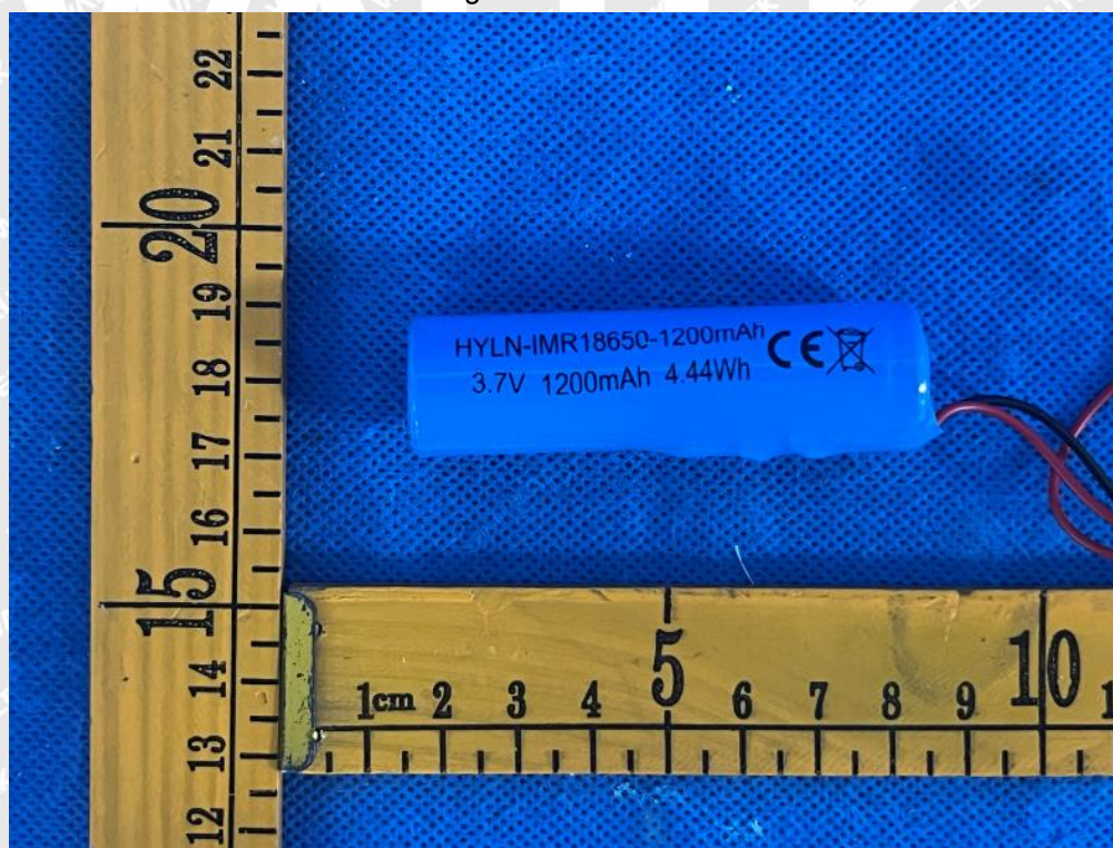
Figure 8: Battery view
