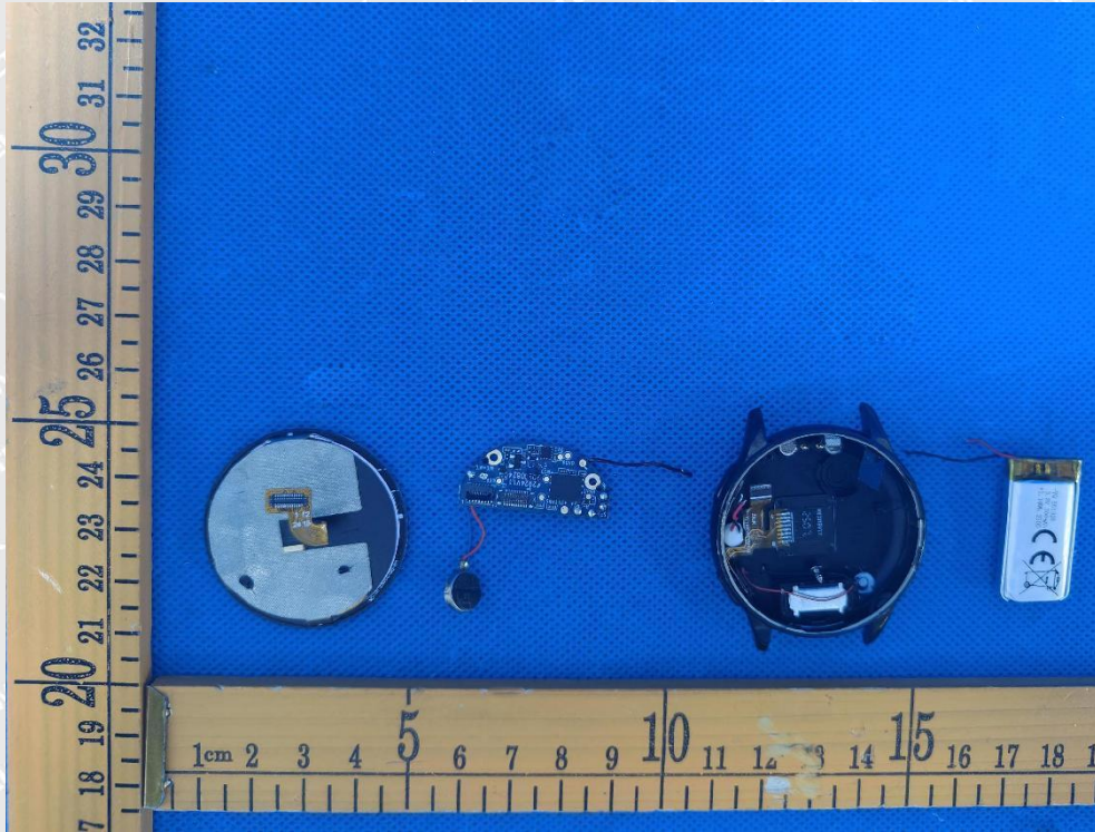
Figure 7: Internal view
