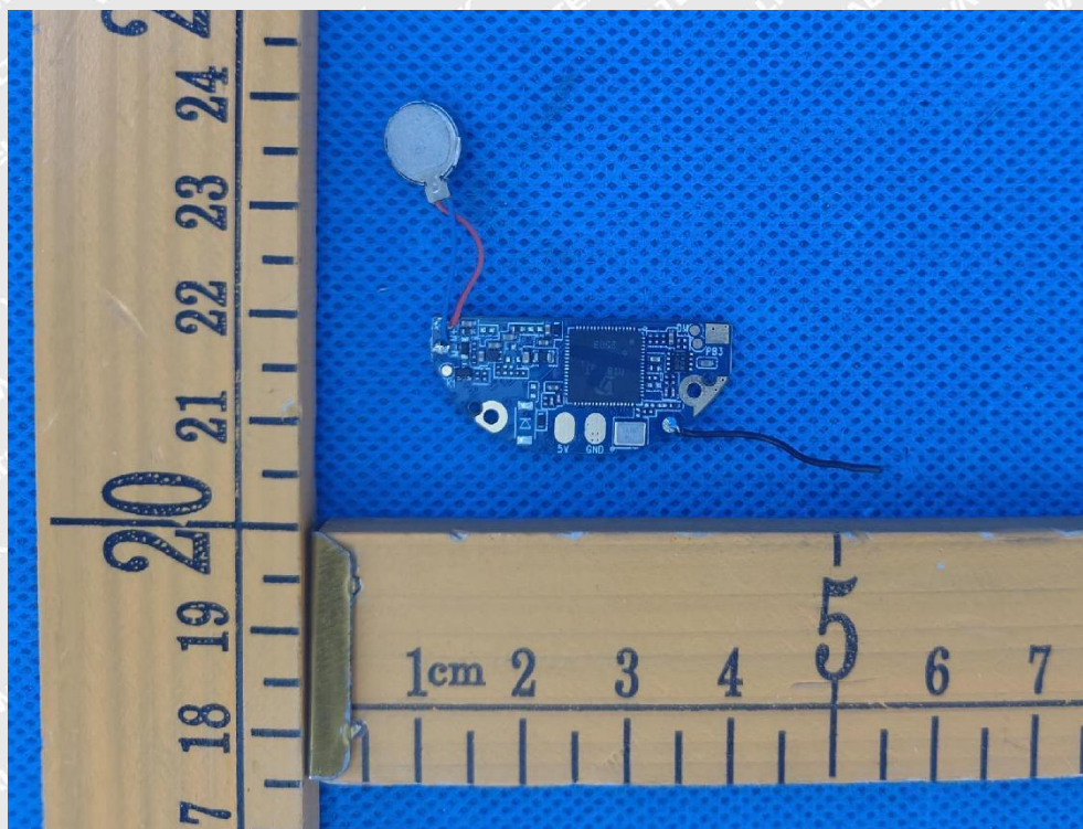
Figure 9: PCB view
