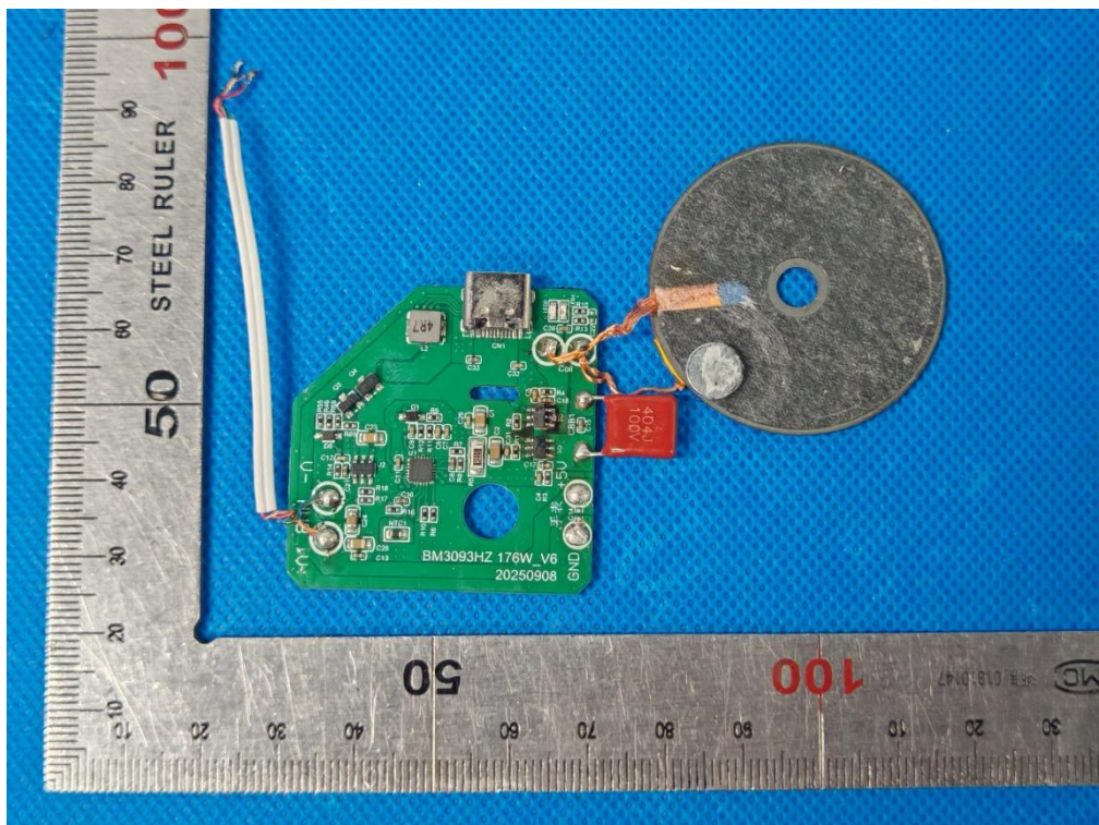
Fig.12 – PCB view
