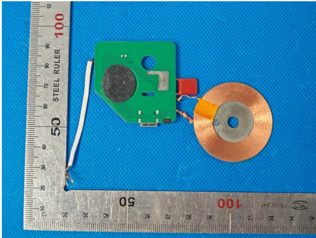
Fig.13 – PCB view
