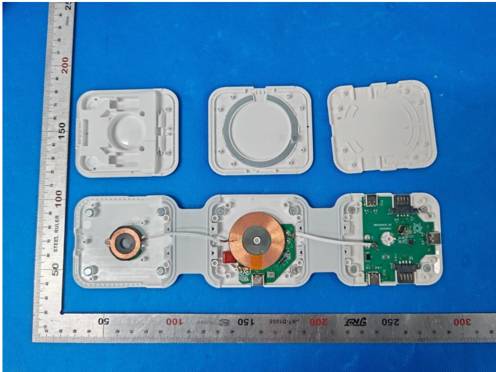
Fig.9 –open view
