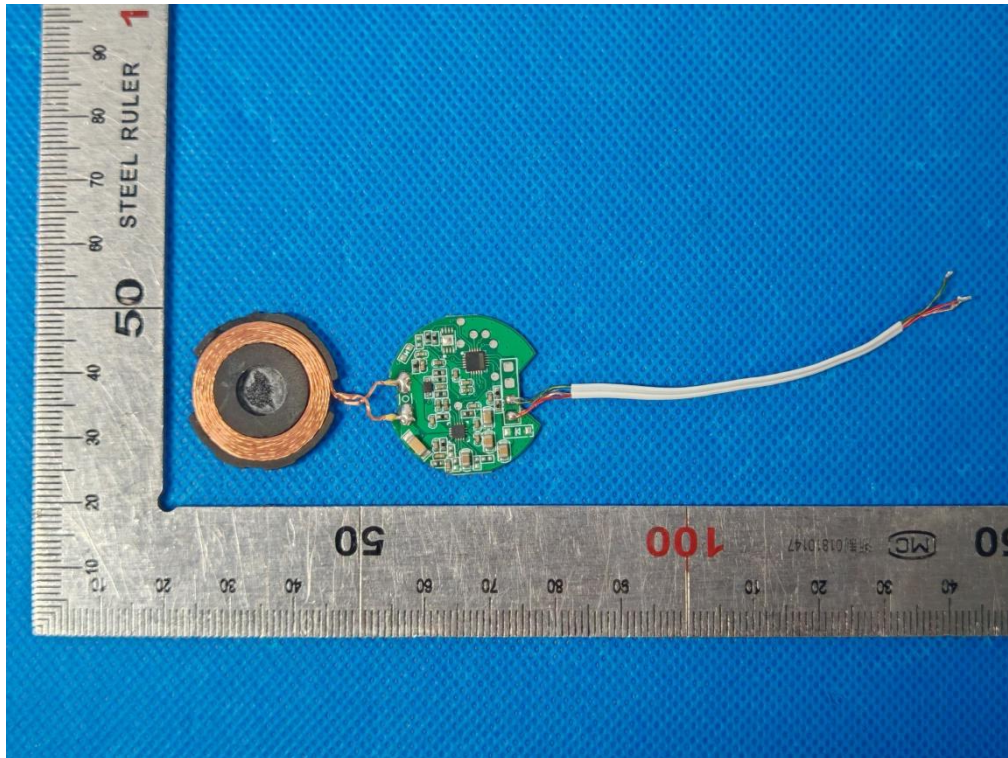
Fig.15 – PCB view
