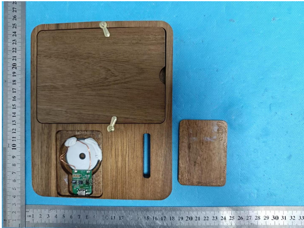
Fig. 5 – Open view
