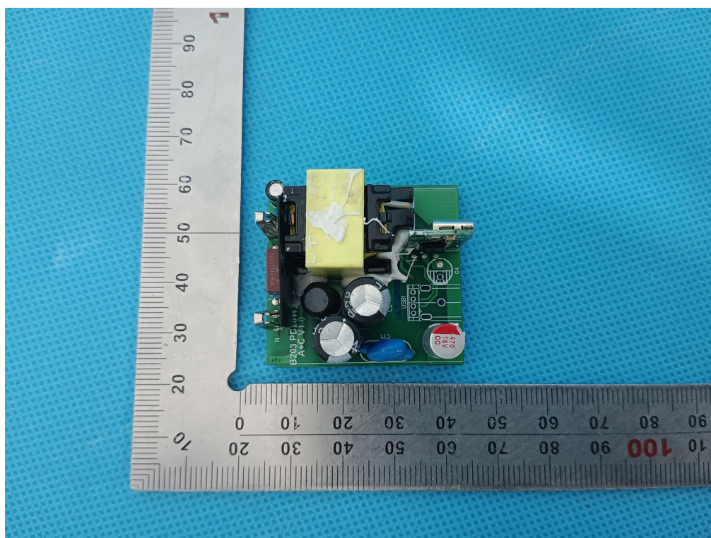
Figure 5: PCB view
