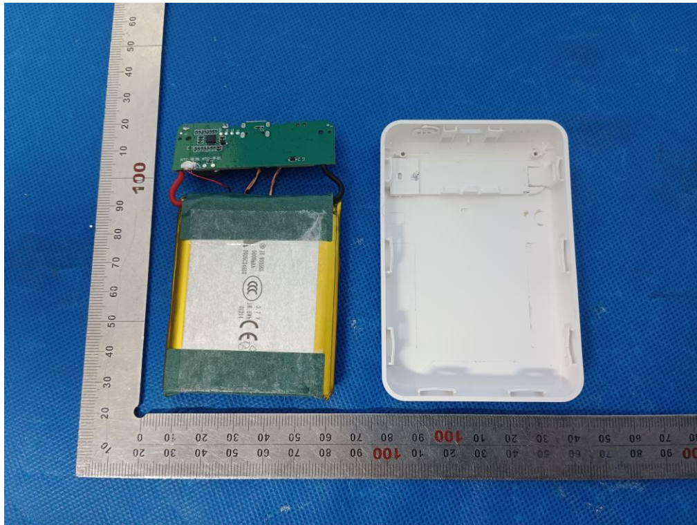
Fig. 5- Internal view
