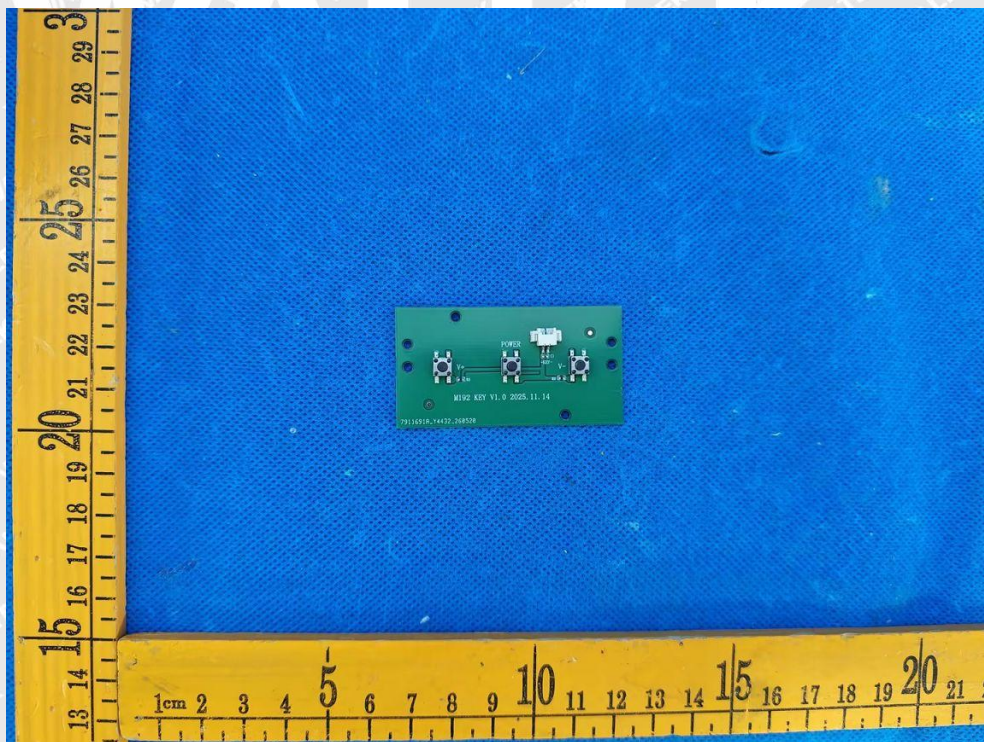
Figure 8: PCB view
