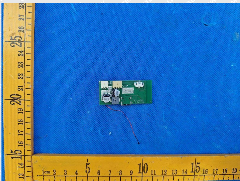
Figure 7: PCB view
