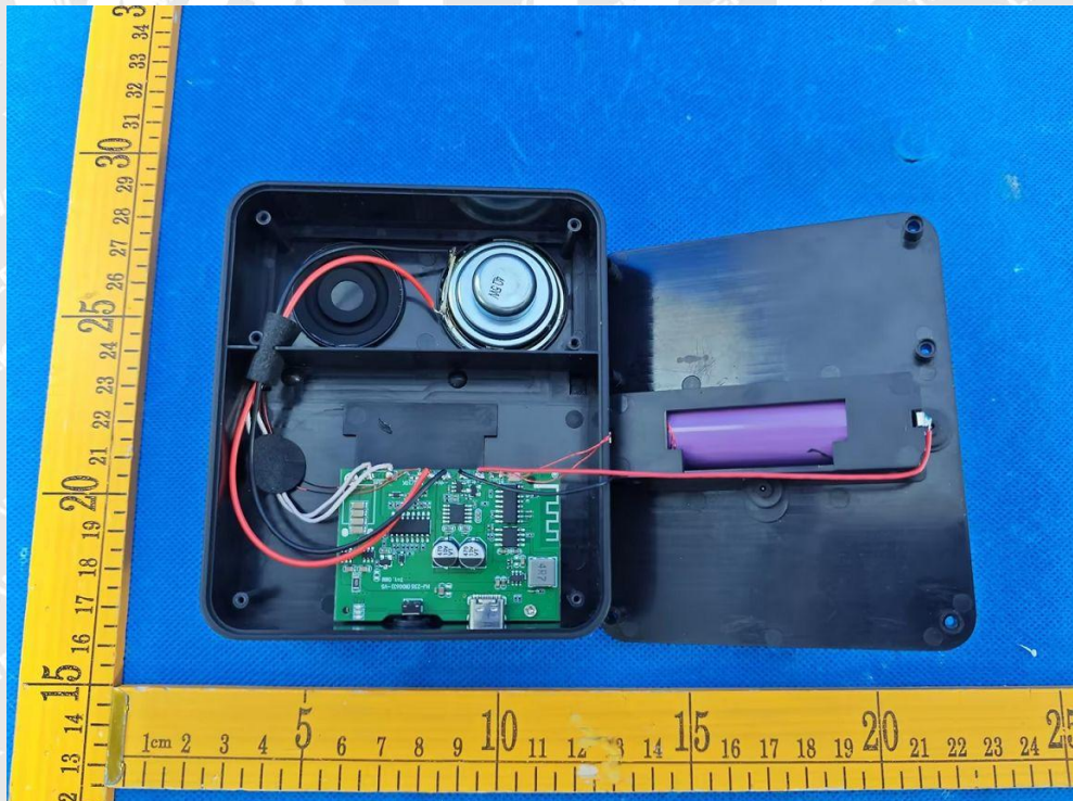
Figure 8: Internal view
