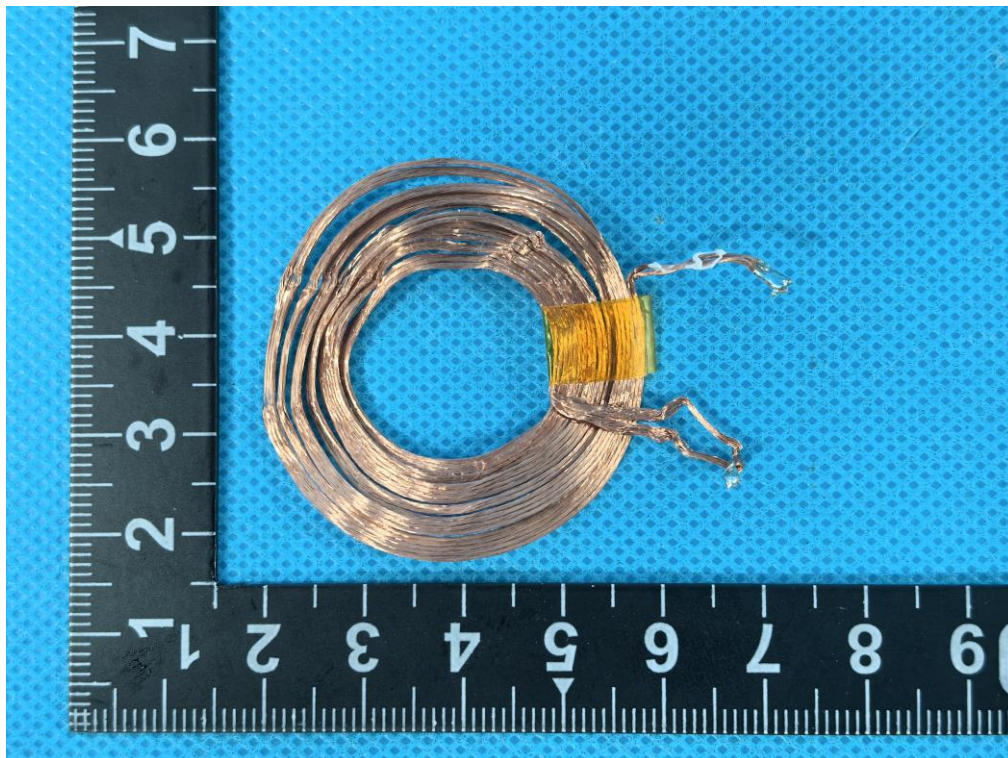
Fig. 12 – Coil view (Earbud)
