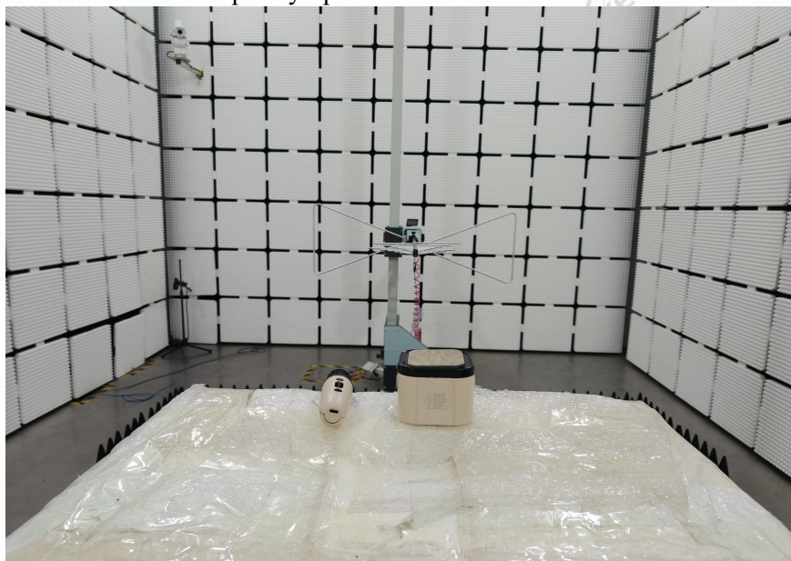
Frequency Spurious (30 MHz to 1 GHz)
