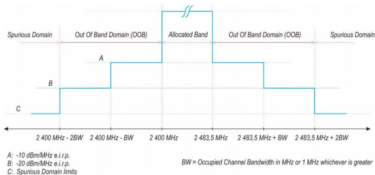
Figure 1: Transmit mask
