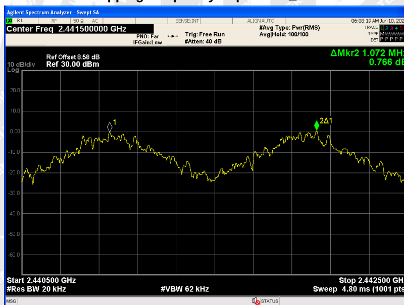
Hopping Frequency Separation_DH5
