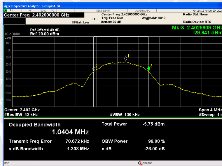
Occupied Channel Bandwidth_NTNV_BLE_2402_1Mbps
