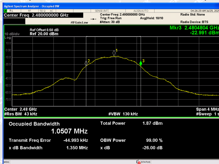
Occupied Channel Bandwidth_NTNV_BLE_2480_1Mbps
