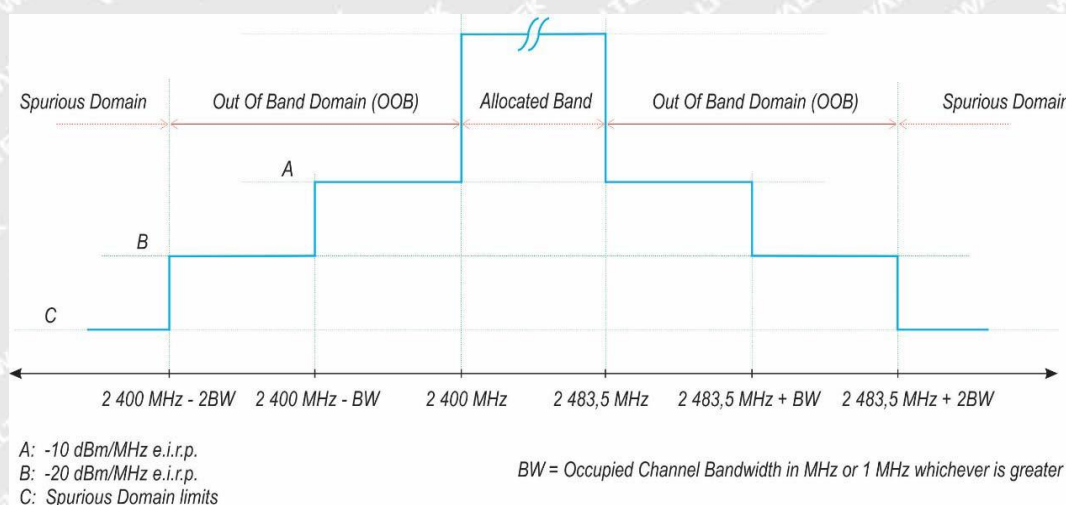
Figure 1: Transmit mask
