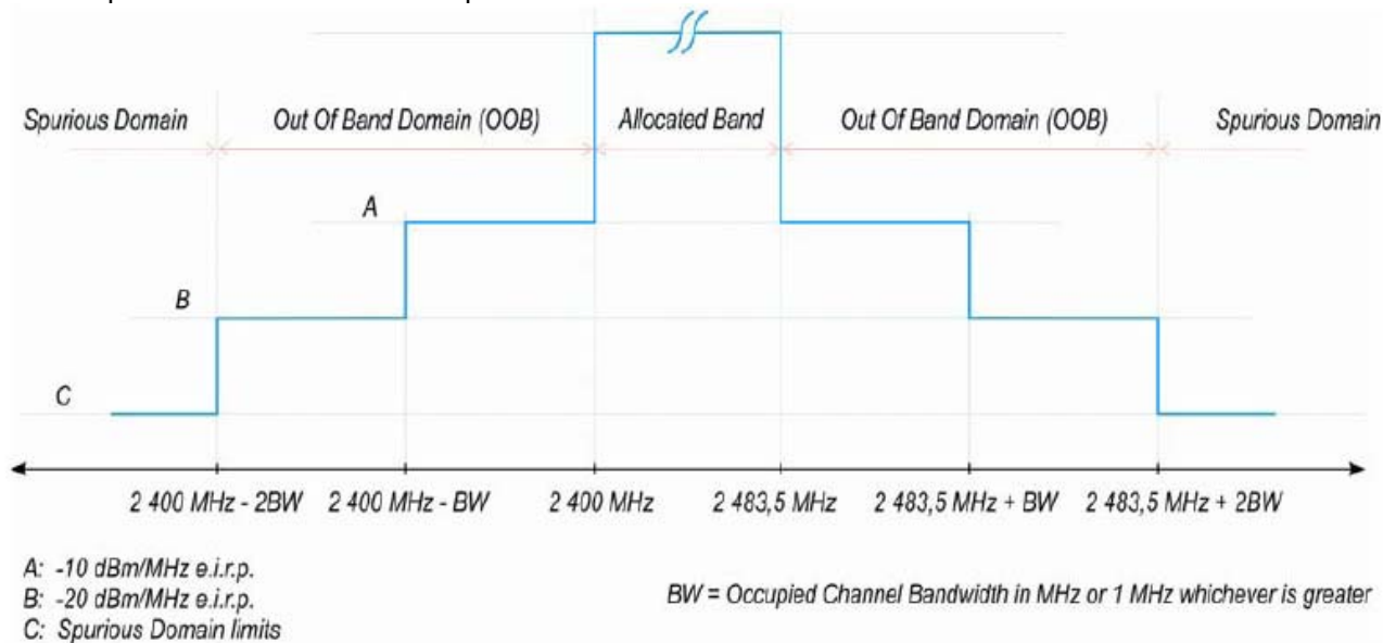
Figure 3: Transmit mask
