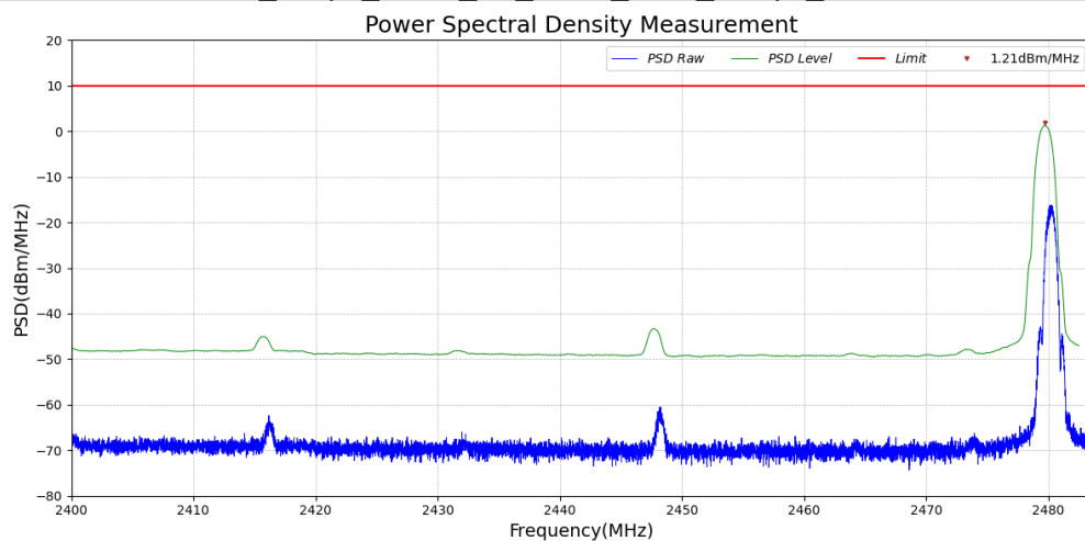
Test_Graph_LE1M_TX_ANT1_2480_1Mbps_PSD
