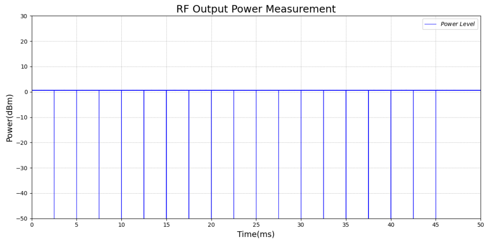
Test_Graph_LE1M_TX_ANT1_2440_1Mbps_Power_HT
