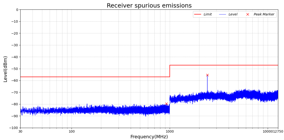
Test_Graph_LE1M_RX_ANT1_2402_1Mbps_RX
