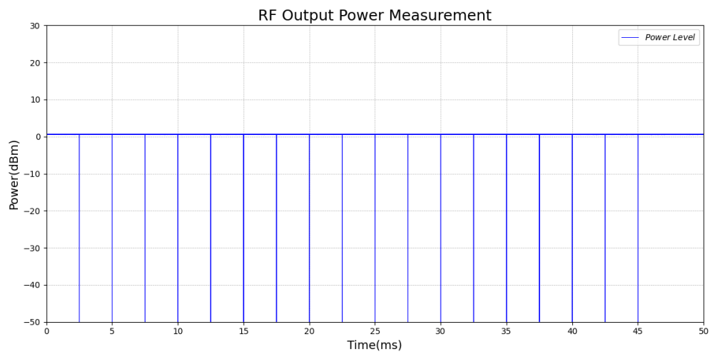
Test_Graph_LE1M_TX_ANT1_2440_1Mbps_Power_NT
