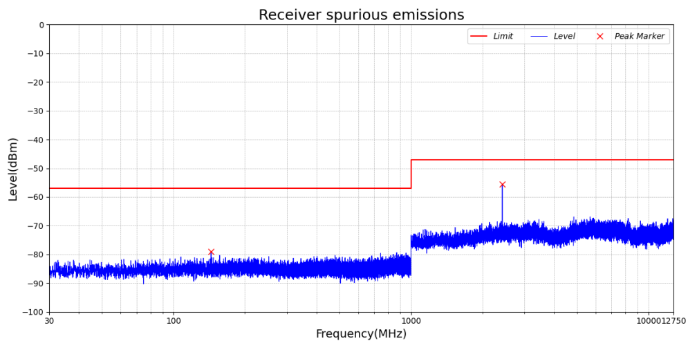
Test_Graph_LE1M_RX_ANT1_2480_1Mbps_RX
