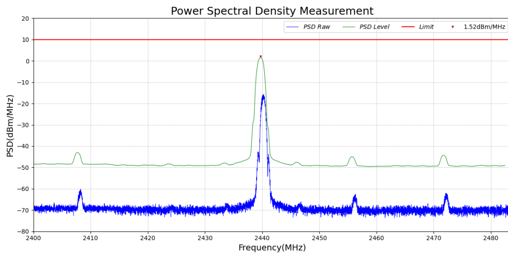
Test_Graph_LE1M_TX_ANT1_2440_1Mbps_PSD
