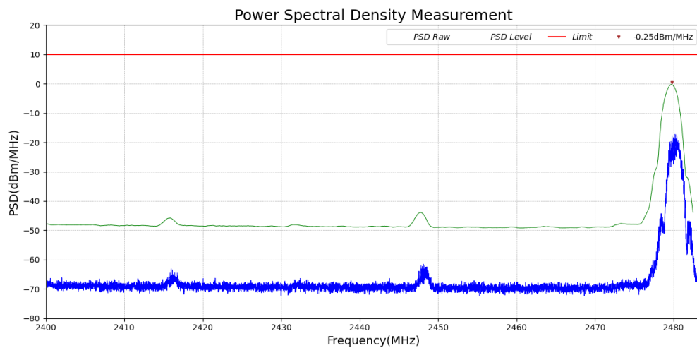
Test_Graph_LE2M_TX_ANT1_2480_2Mbps_PSD
