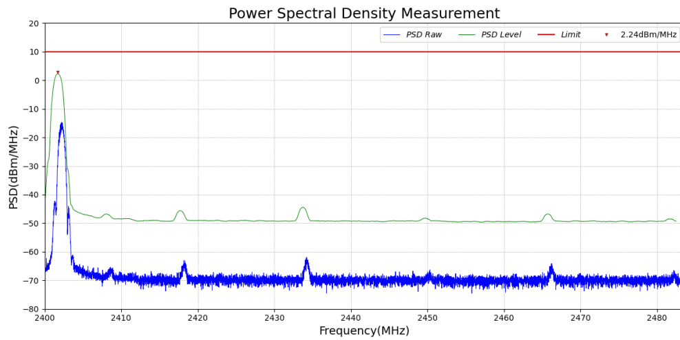
Test_Graph_LE1M_TX_ANT1_2402_1Mbps_PSD
