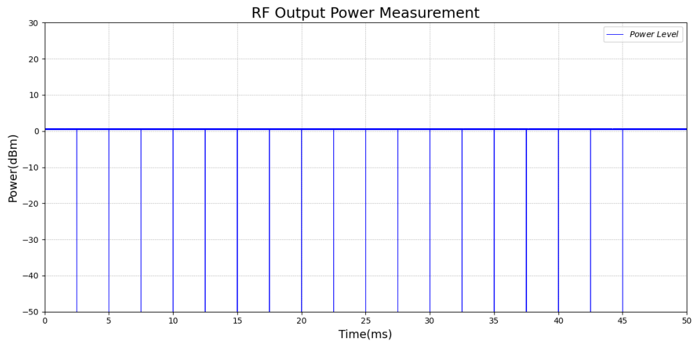
Test_Graph_LE2M_TX_ANT1_2440_2Mbps_Power_HT
