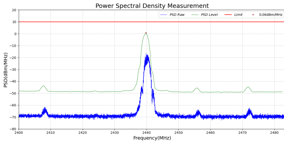
Test_Graph_LE2M_TX_ANT1_2440_2Mbps_PSD
