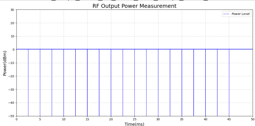
Test_Graph_LE1M_TX_ANT1_2480_1Mbps_Power_NT
