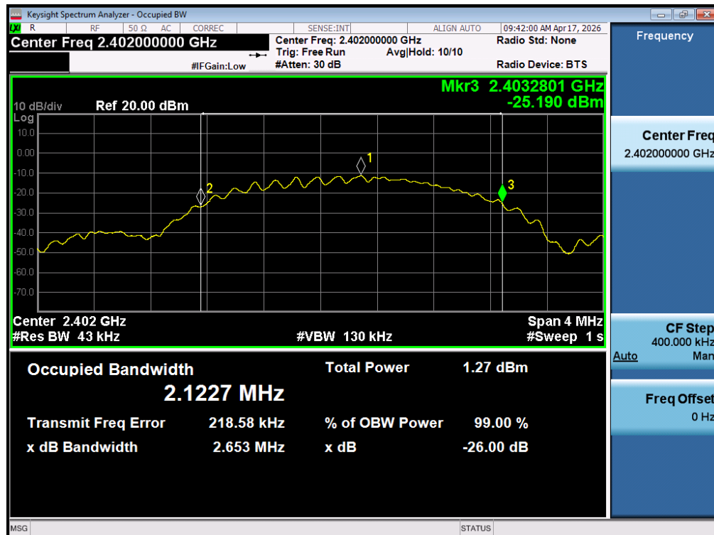
Test Graph LE2M TX ANT1 2402 2Mbps OBW
