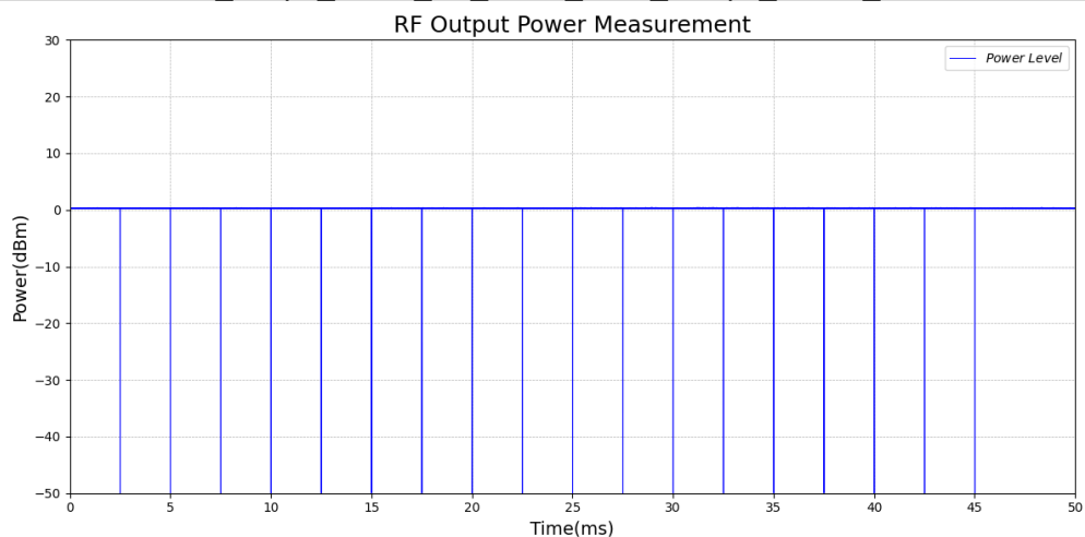
Test_Graph_LE1M_TX_ANT1_2480_1Mbps_Power_LT
