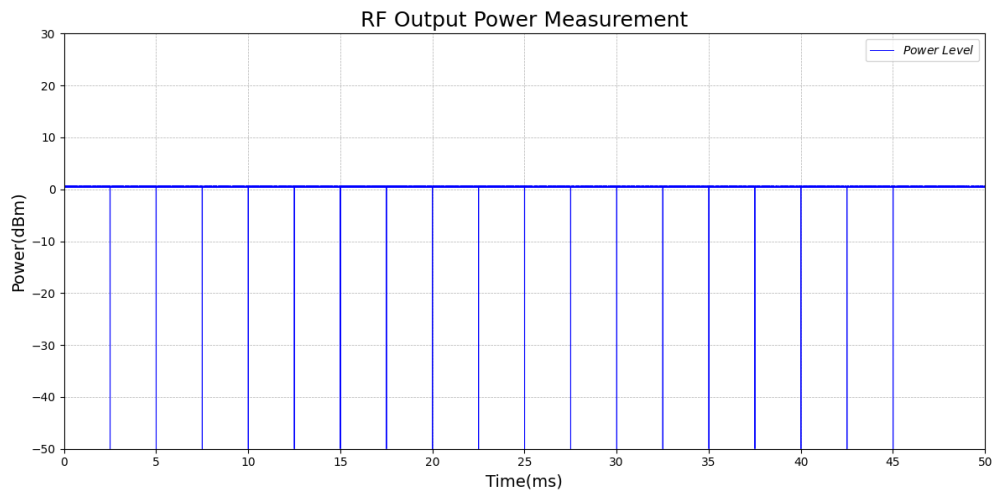
Test_Graph_LE2M_TX_ANT1_2440_2Mbps_Power_NT
