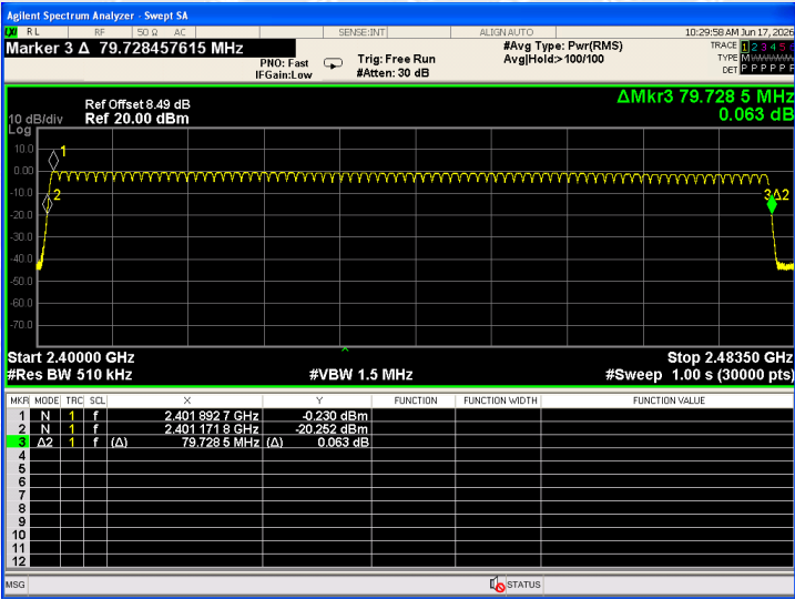
Hopping Sequence_DH5
