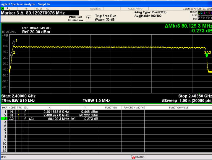
Hopping Sequence_2DH5
