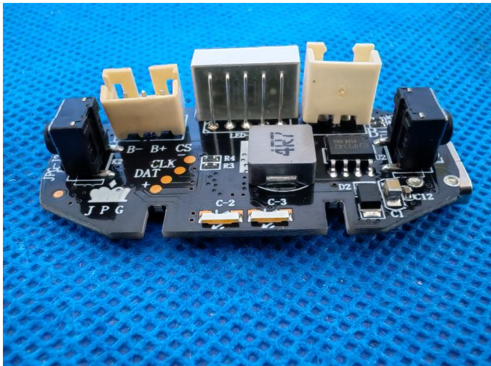
Fig.6- Part view
