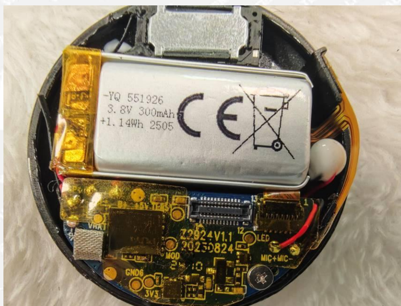
Photo 6 -- After the test of IP6X
