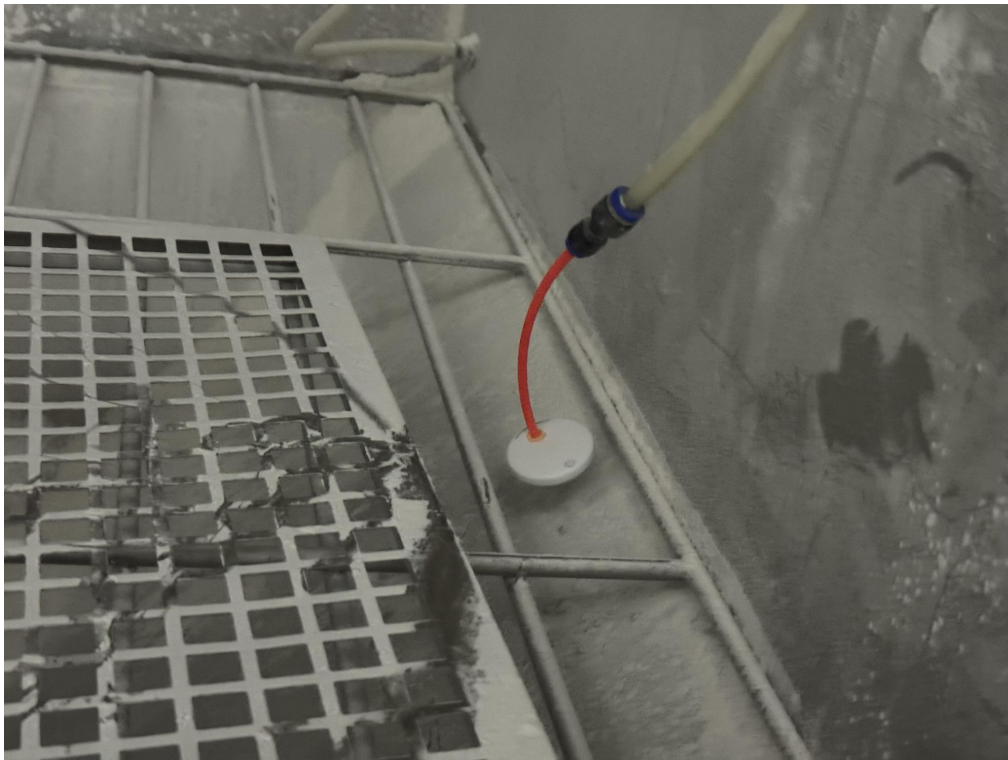
Fig.3 – View of product during test (IP6X)
