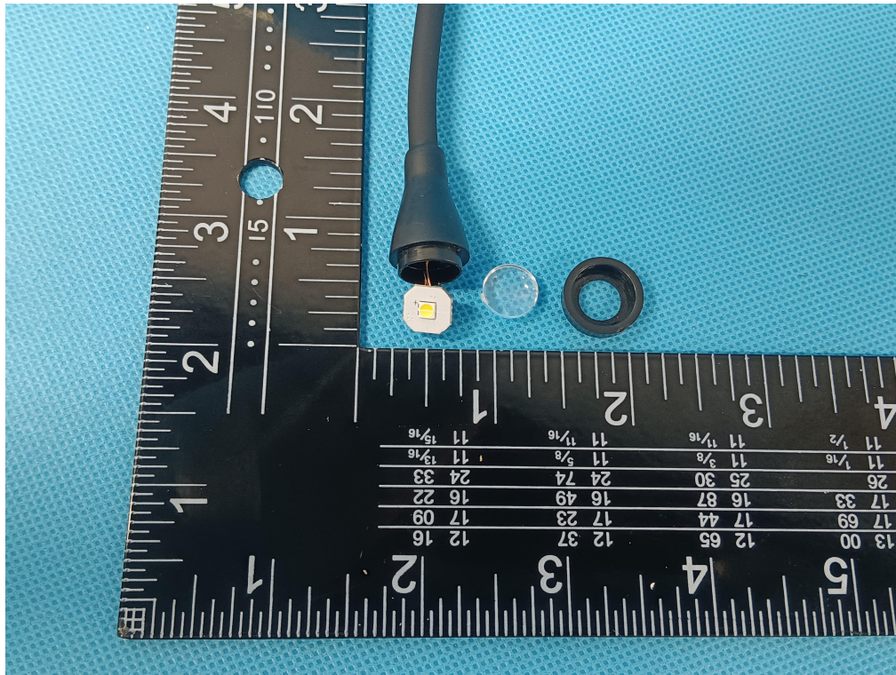
Fig.6– Parts view
